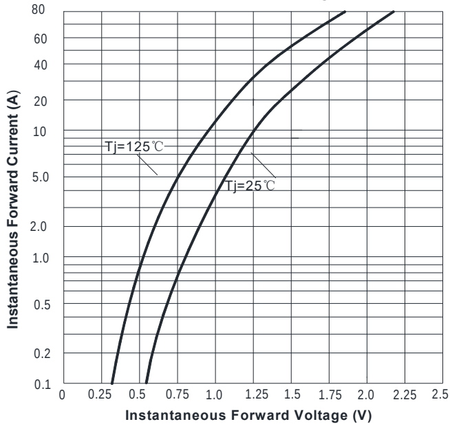
FIG3: Forward Voltage
